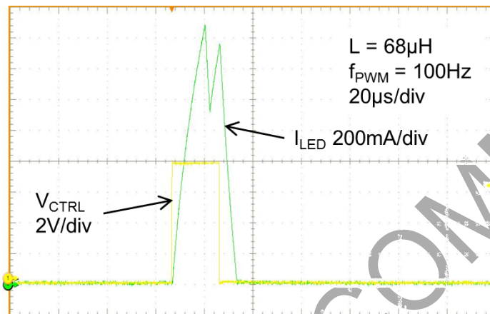
Figure 36. 0.2% PWM Duty Cycle at 100Hz PWM Frequency and 68μH Inductance
