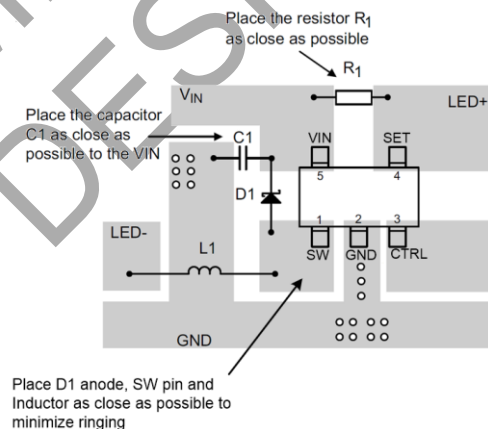
Figure 44. Recommended PCB Layout
