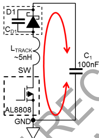
Figure 43. PCB Loop Resonance
