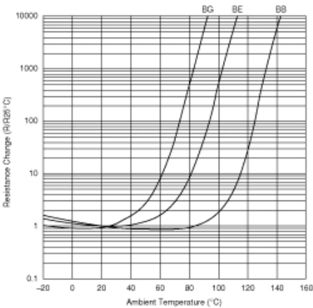
Resistance-Temperature Characteristics
