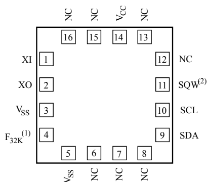
Figure 5. M41T64 connections
