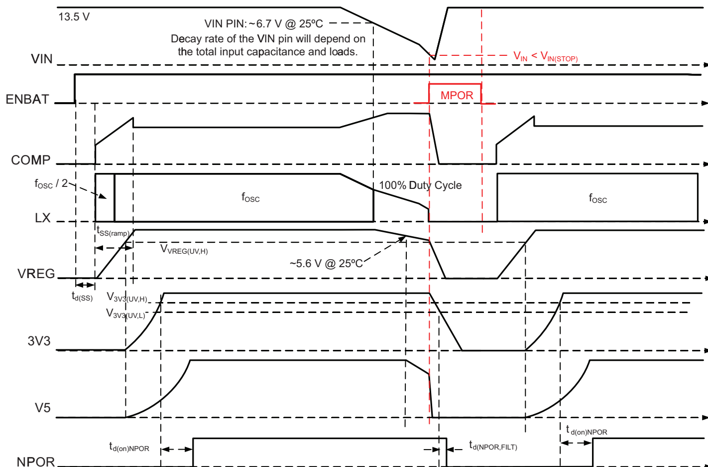
Figure 3: Input Undervoltage Timing, when V_{IN} < V_{IN(STOP)}
