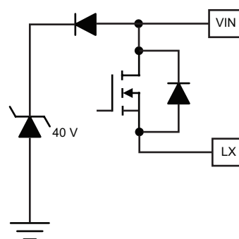
Figure 20: VIN, LX
