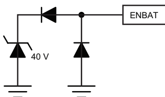
Figure 21: ENBAT
