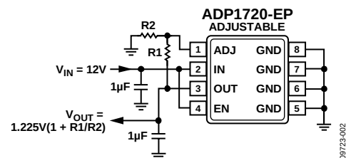
Figure 2. ADP1720-EP with Adjustable Output Voltage, 1.225 V to 5.0 V
