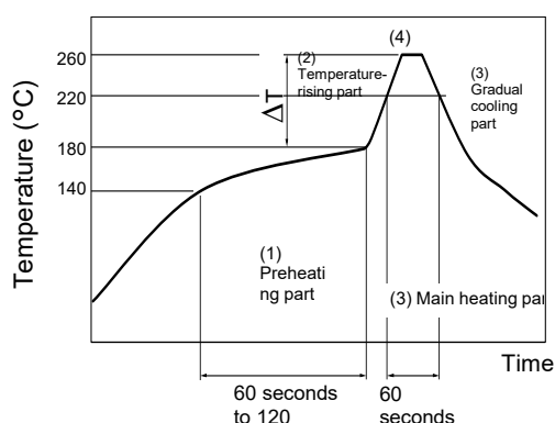
Recommended reflow soldering profile (example)
