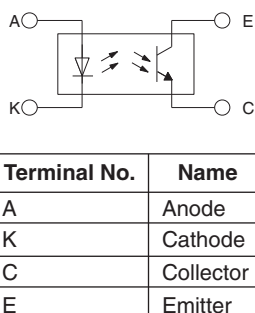
Internal Circuit
