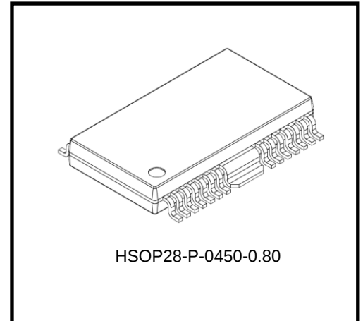
Weight: 0.79 g (typ.)
