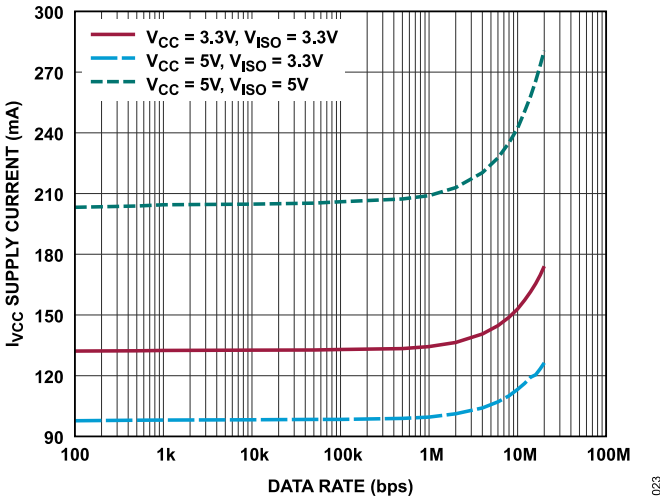
Figure 23. V CC Supply Current vs. Frequency, T A = 25°C, (ADM2895E-1), 54Ω Termination, Logarithmic Scale
