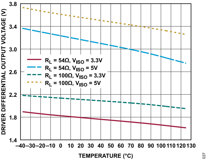
Figure 37. Driver Differential Output Voltage vs. Temperature
