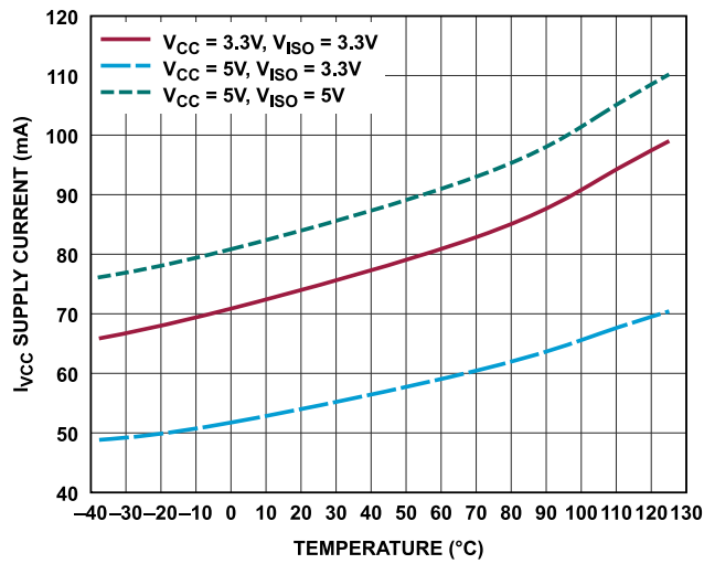
Figure 9. V_{CC} Supply Current vs. Temperature at 250kbps (ADM2895E), Unterminated Bus
