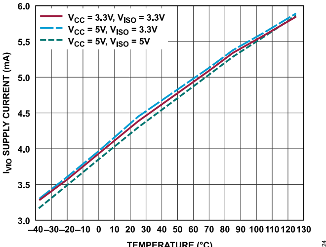
Figure 24. V IO Supply Current vs. Temperature at 250kbps (ADM2895E), Underterminated Bus
