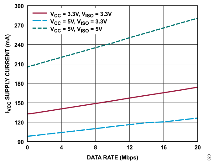
Figure 20. V_{CC} Supply Current vs. Frequency, T_A = 25^\circ\text{C} , (ADM2895E-1), 54Ω Termination, Linear Scale
