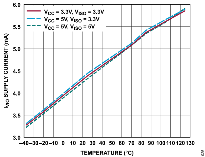
Figure 25. V_{I0} Supply Current vs. Temperature at 250kbps (ADM2895E), 120Ω Termination
