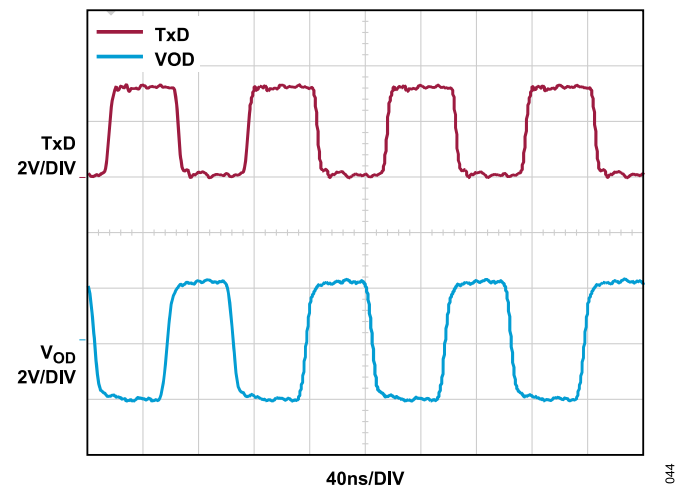
Figure 44. Driver Switching at 20Mbps, (ADM2895E-1)
