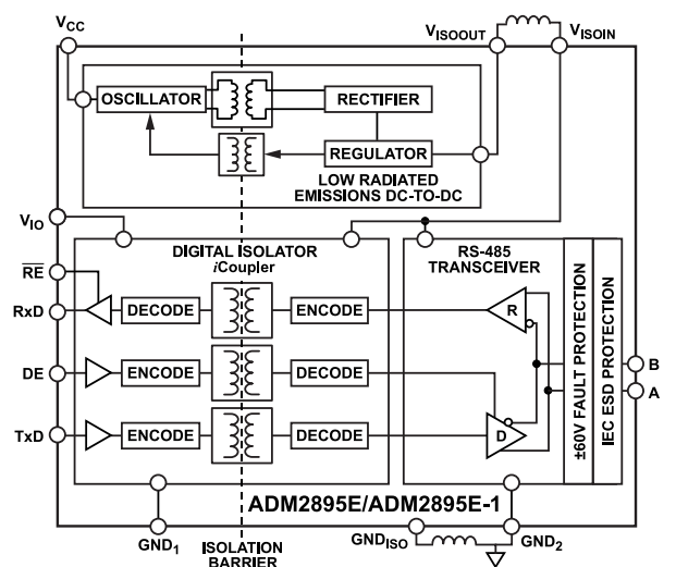
Figure 1. ADM2895E/ADM2895E-1 Functional Block Diagram
