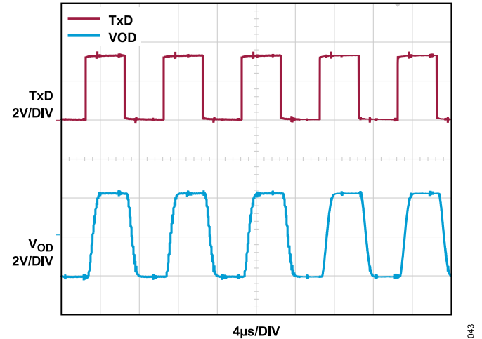
Figure 43. Driver Switching at 250kbps, (ADM2895E)
