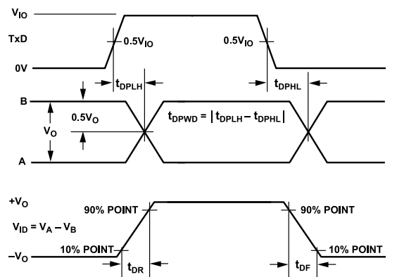
Figure 2. Driver Propagation Delay, Rise/Fall Timing
