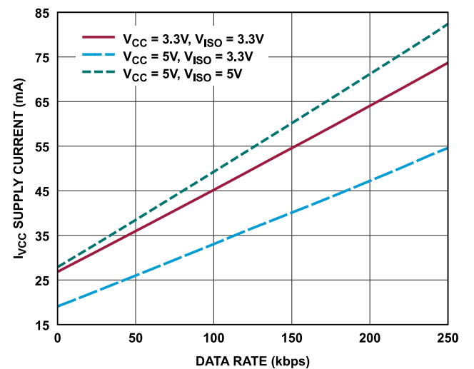
Figure 12. V_{CC} Supply Current vs. Frequency, T_A = 25^\circ\text{C} , (ADM2895E), Unterminated Bus
