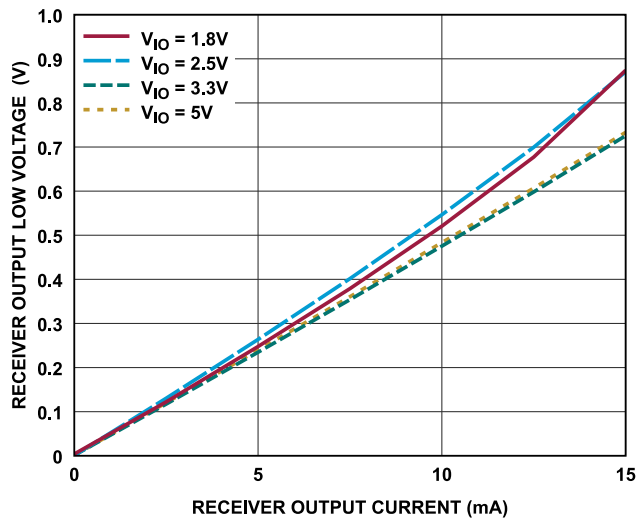
Figure 46. Receiver Output Low Voltage vs. Receiver Output Current
