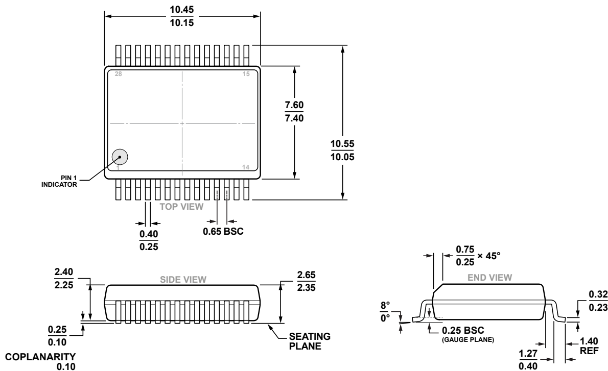
Figure 67. 28-Lead Standard Small Outline, Wide Body, with Finer Pitch [SOIC_W_FP] (RN-28-1) Dimensions Shown in millimeters
