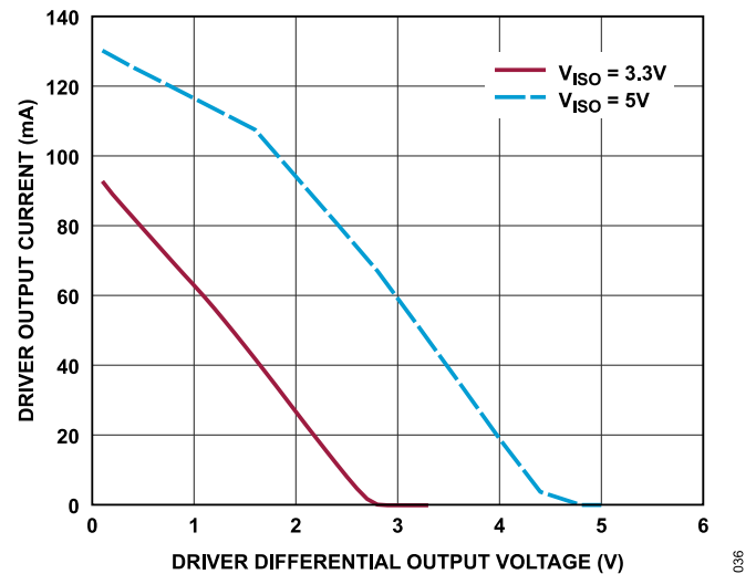
Figure 36. Driver Output Current vs. Driver Differential Output Voltage
