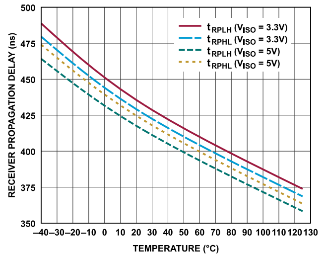
Figure 49. Receiver Propagation Delay vs. Temperature
