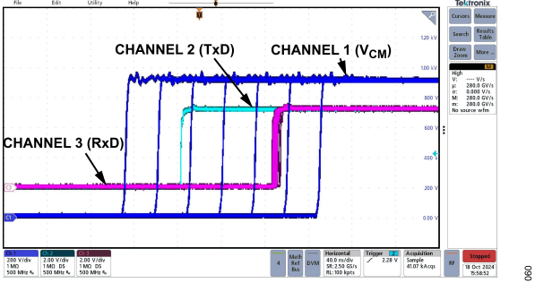
Figure 60. Switching Correctly in the Presence of >250V/ns Common-Mode Transients
