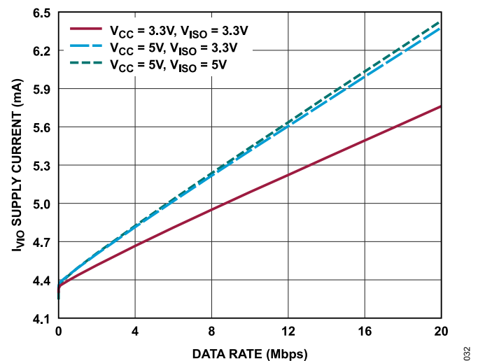
Figure 32. I_{VIO} Supply Current vs. Data Rate, T_A = 25^\circ\text{C} , (ADM2895E-1), 54 \Omega Termination, Linear Scale
