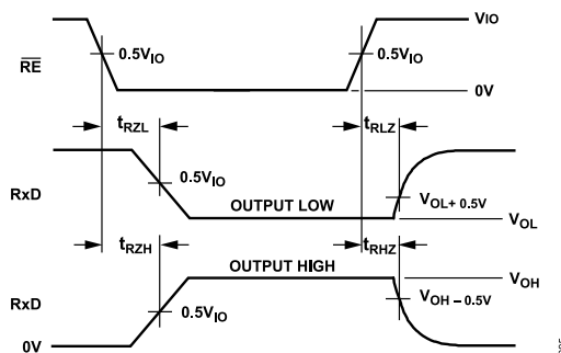
Figure 5. Receiver Enable or Disable Timing
