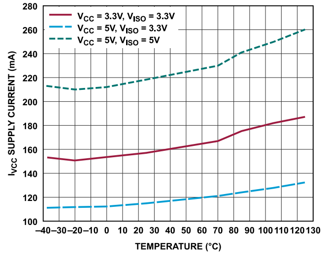
Figure 11. V_{CC} Supply Current vs. Temperature at 250kbps (ADM2895E), 54Ω Termination
