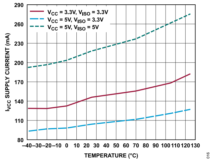
Figure 16. V_{CC} Supply Current vs. Temperature at 20Mbps (ADM2895E-1), 120 \Omega Termination
