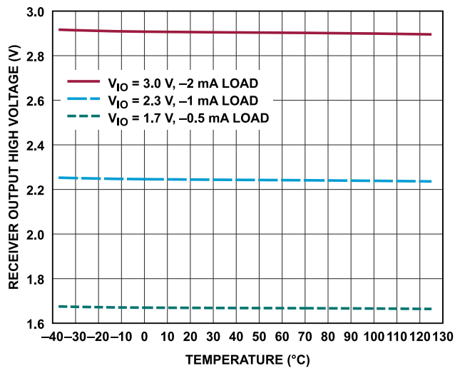
Figure 47. Receiver Output High Voltage vs. Temperature
