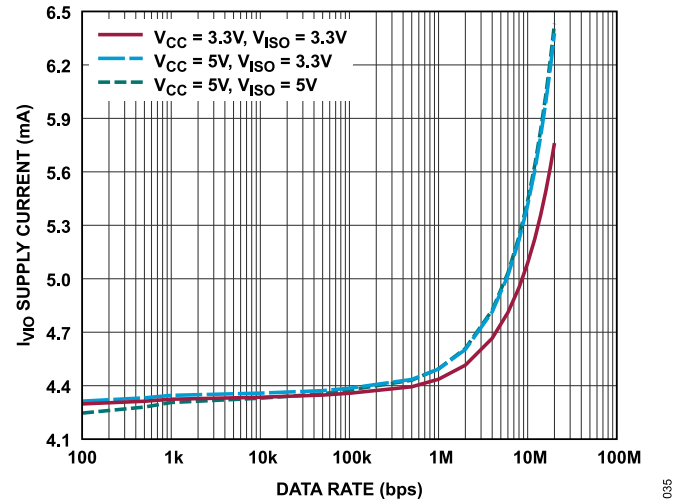
Figure 35. I_{VIO} Supply Current vs. Data Rate, T_A = 25^\circ\text{C} , (ADM2895E-1), 54\Omega termination, Logarithmic Scale
