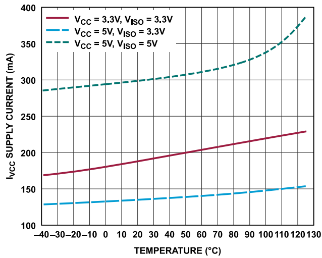
Figure 17. V_{CC} Supply Current vs. Temperature at 20Mbps (ADM2895E-1), 54Ω Termination
