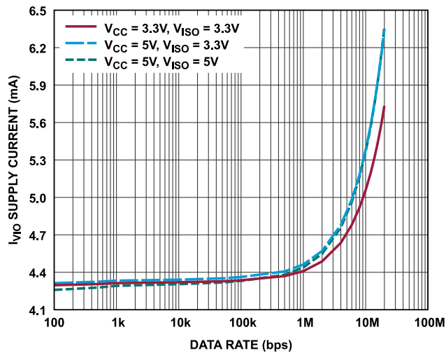
Figure 34. I_{VIO} Supply Current vs. Data Rate, T_A = 25^\circ\text{C} , (ADM2895E-1), 120\Omega Termination, Logarithmic Scale
