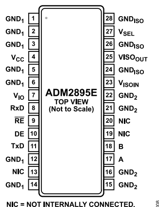
Figure 8. ADM2895E/ADM2895E-1 Pin Configuration
