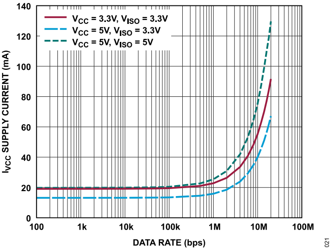
Figure 21. V CC Supply Current vs. Frequency, T A = 25°C, (ADM2895E-1), Underterminated Bus, Logarithmic Scale
