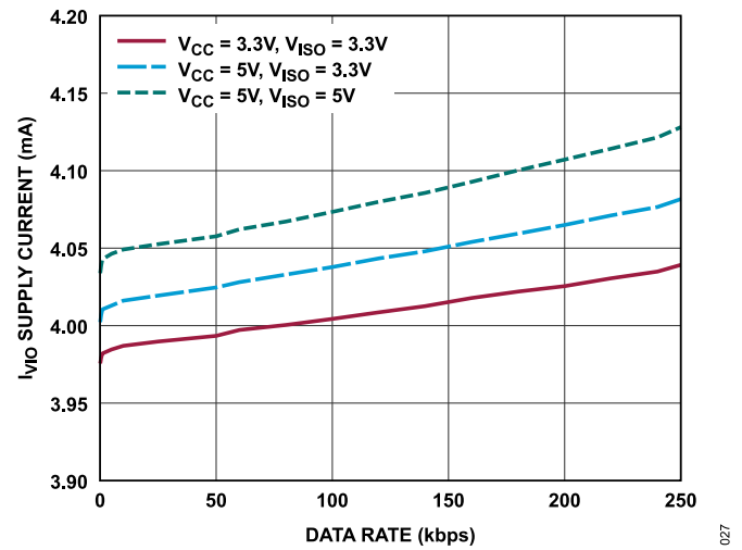
Figure 27. V_{I0} Supply Current vs. Data Rate, T_A = 25^\circ\text{C} , (ADM2895E), Unterminated Bus
