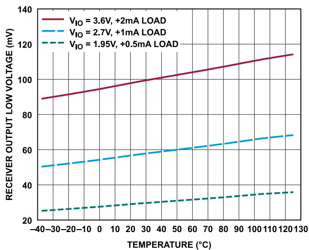
Figure 48. Receiver Output Low Voltage vs. Temperature
