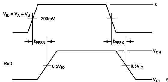
Figure 6. Fail-Safe Entry or Exit Delay Timing
