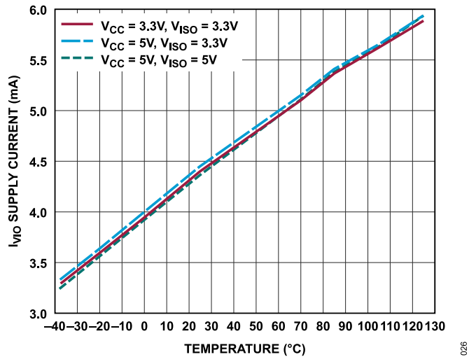
Figure 26. V_{I0} Supply Current vs. Temperature at 250kbps (ADM2895E), 54Ω Termination
