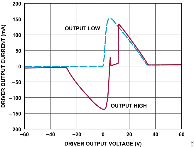
Figure 38. Driver Output Current vs. Driver Output Voltage
