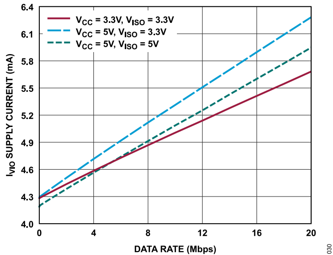
Figure 30. I_{VIO} Supply Current vs. Data Rate, T_A = 25^\circ\text{C} , (ADM2895E-1), Unterminated Bus, Linear Scale
