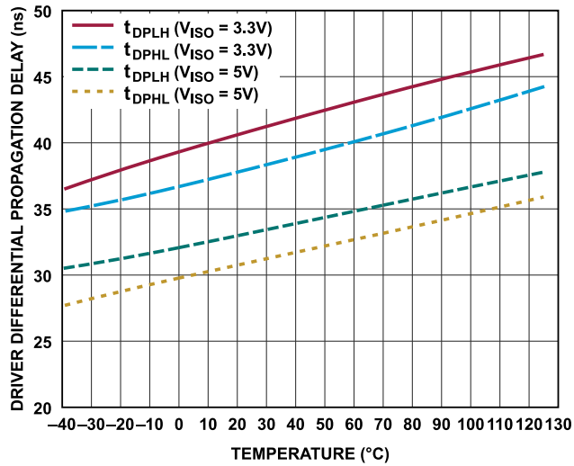
Figure 41. Driver Differential Propagation Delay vs. Temperature, 54Ω Termination (ADM2895E-1)
