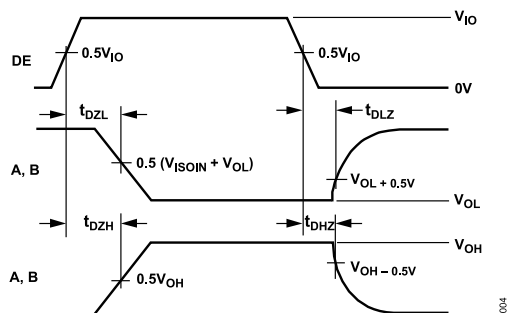
Figure 4. Driver Enable or Disable Timing
