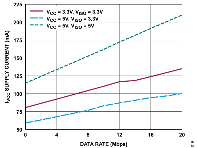
Figure 19. V_{CC} Supply Current vs. Frequency, T_A = 25^\circ\text{C} , (ADM2895E-1), 120Ω Termination, Linear Scale
