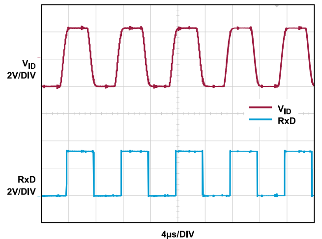
Figure 50. Receiver Switching at 250kbps, (ADM2895E)
