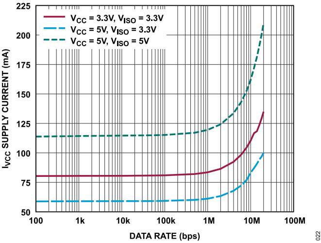
Figure 22. V CC Supply Current vs. Frequency, T A = 25°C, (ADM2895E-1), 120Ω Termination, Logarithmic Scale
