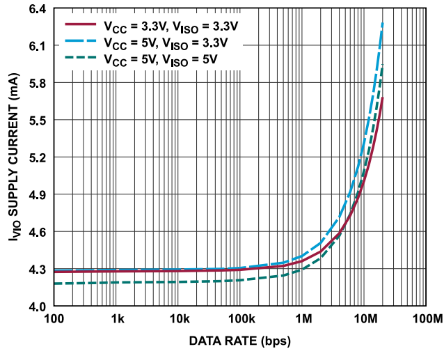
Figure 33. I_{VIO} Supply Current vs. Data Rate, T_A = 25^\circ\text{C} , (ADM2895E-1), Underterminated Bus, Logarithmic Scale
