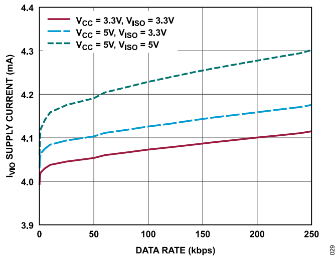
Figure 29. I_{VIO} Supply Current vs. Data Rate, T_A = 25^\circ\text{C} , (ADM2895E), 54 \Omega Termination
