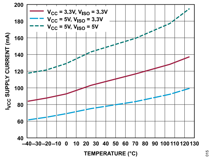
Figure 15. V_{CC} Supply Current vs. Temperature at 20Mbps (ADM2895E-1), Unterminated Bus
