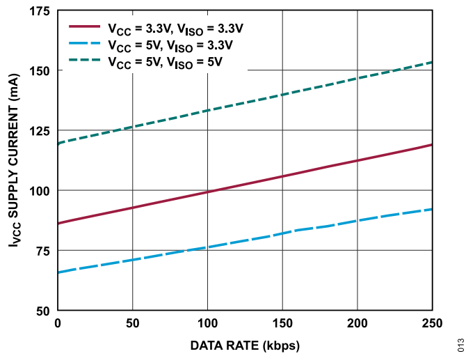
Figure 13. V_{CC} Supply Current vs. Frequency, T_A = 25^\circ\text{C} , (ADM2895E), 120 \Omega Termination
