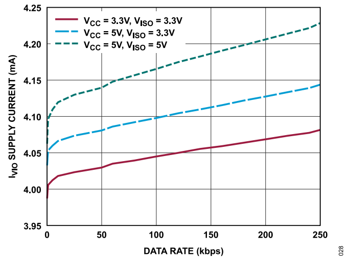
Figure 28. V_{I0} Supply Current vs. Data Rate, T_A = 25^\circ\text{C} , (ADM2895E), 120Ω Termination
