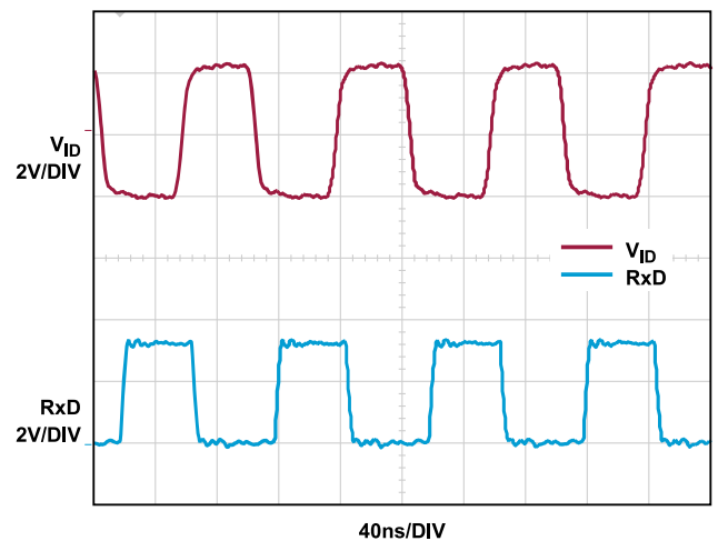
Figure 51. Receiver Switching at 20Mbps, (ADM2895E-1)
