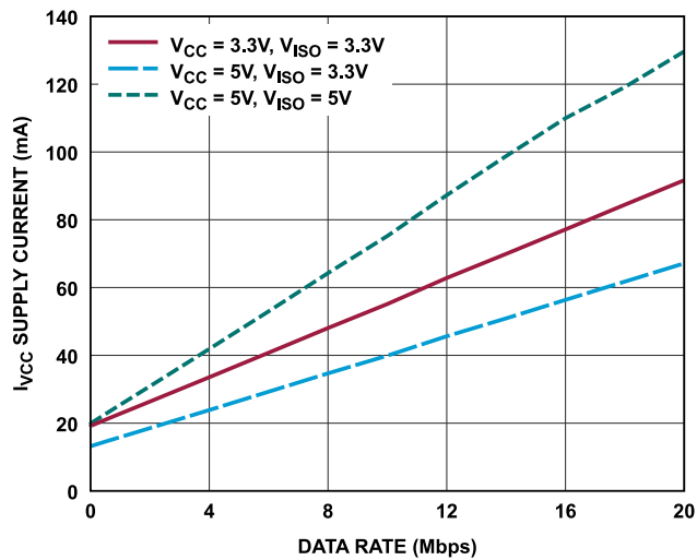
Figure 18. V_{CC} Supply Current vs. Frequency, T_A = 25^\circ\text{C} , (ADM2895E-1), Unterminated Bus, Linear Scale
