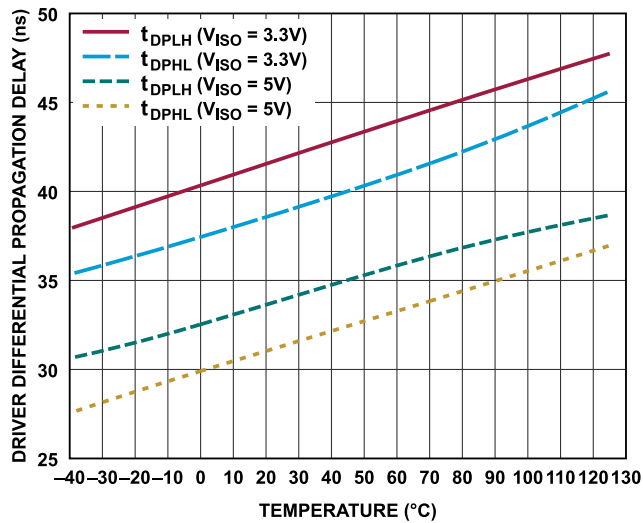
Figure 42. Driver Differential Propagation Delay vs. Temperature, 100Ω Termination (ADM2895E-1)
