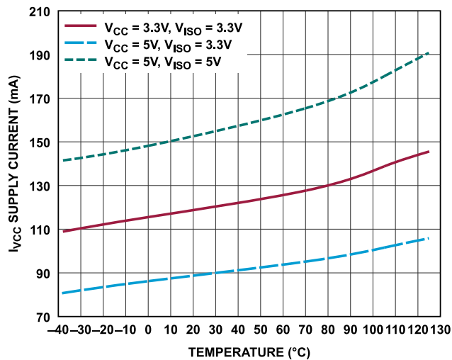
Figure 10. V_{CC} Supply Current vs. Temperature at 250kbps (ADM2895E), 120Ω Termination
