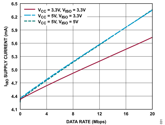
Figure 31. I_{VIO} Supply Current vs. Data Rate, T_A = 25^\circ\text{C} , (ADM2895E-1), 120 \Omega Termination, Linear Scale
