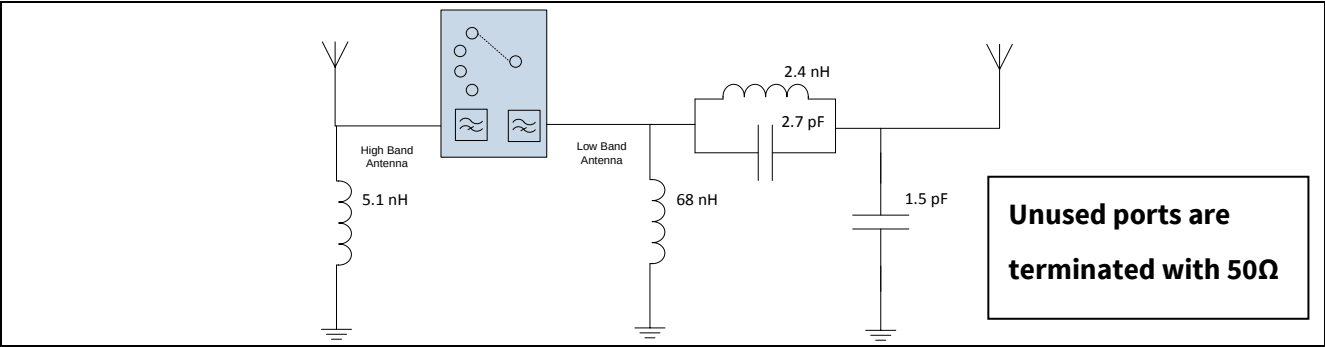
Figure 11 Application circuit BGSF1717MN26
