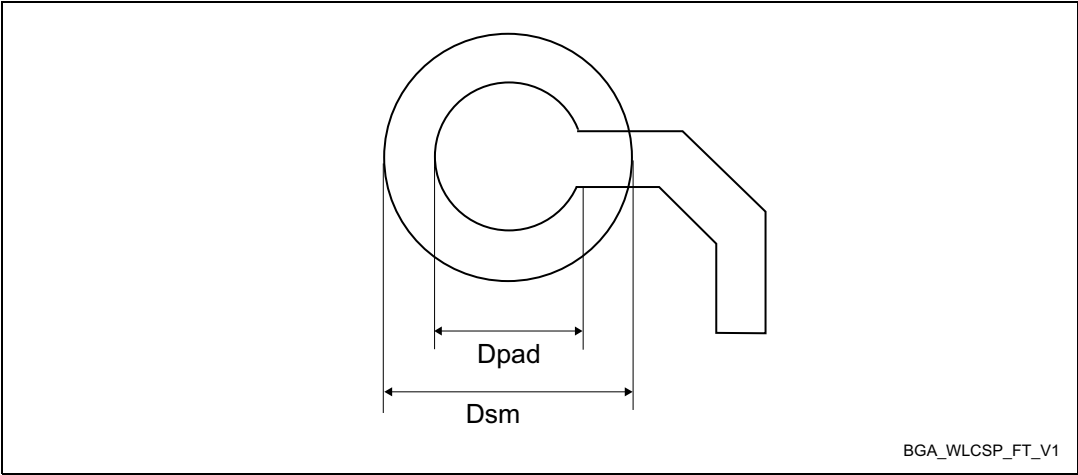
Figure 86. UFBGA169 - Footprint example
