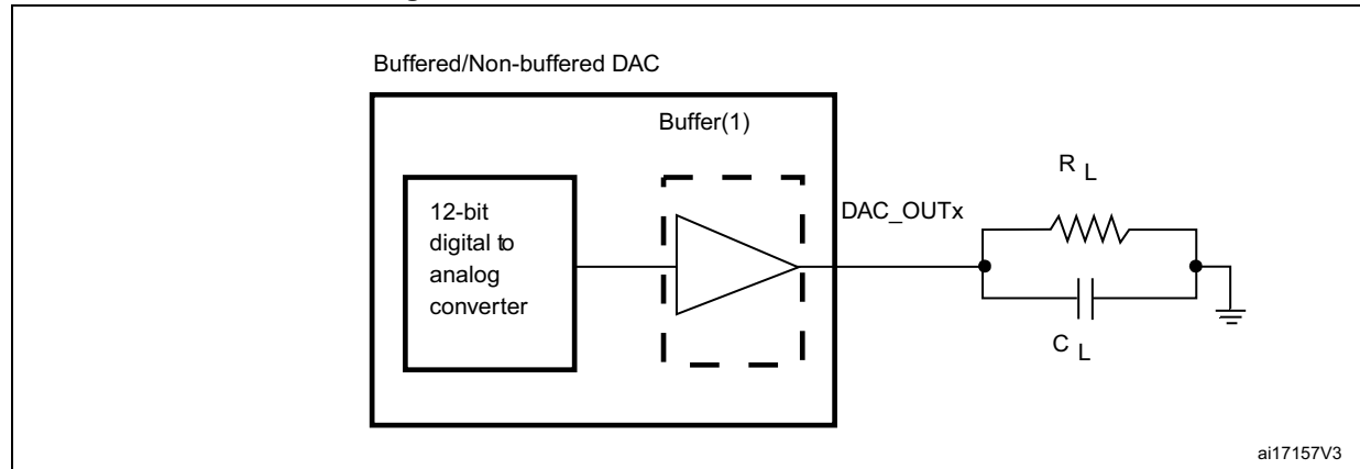
Figure 48. 12-bit buffered /non-buffered DAC
