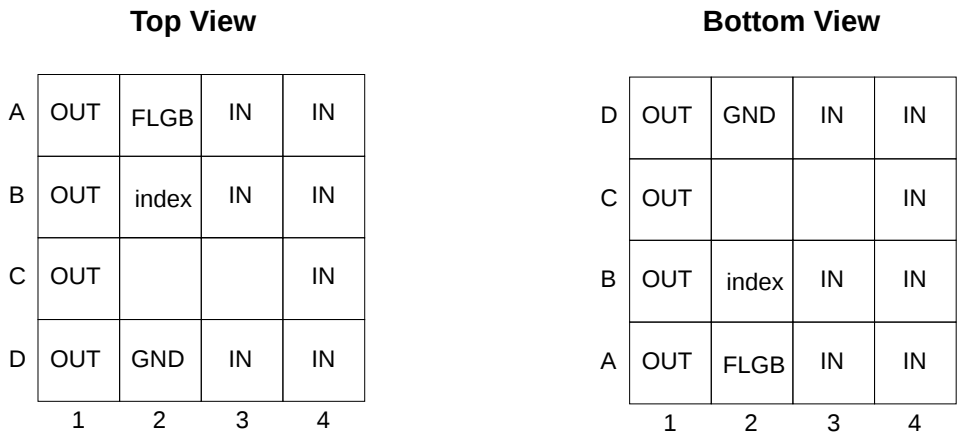
Fig. 3 Ball Configuration
