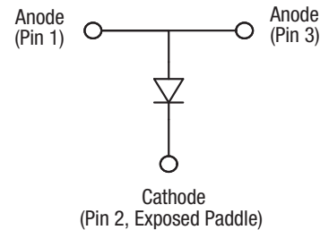
Figure 1. CLA4611-085LF Block Diagram
