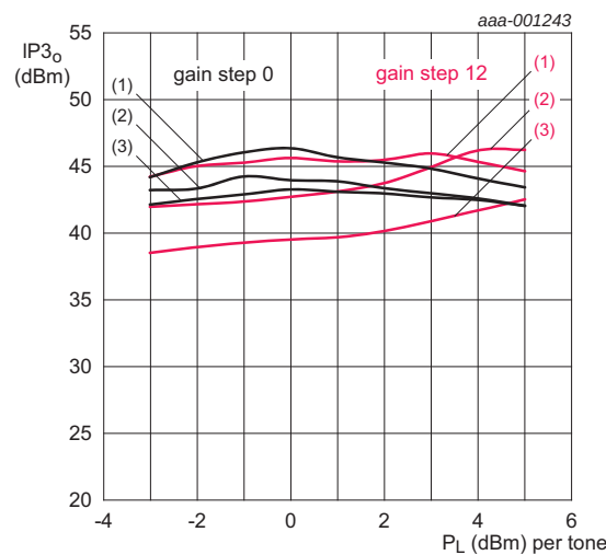
Tuned for f_{IF} = 172 MHz. (1) T_{amb} = -40 °C (2) T_{amb} = +25 °C (3) T_{amb} = +85 °C
