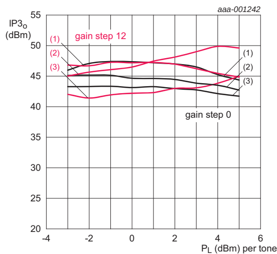
Tuned for f_{IF} = 140 MHz. (1) T_{amb} = -40 °C (2) T_{amb} = +25 °C (3) T_{amb} = +85 °C
