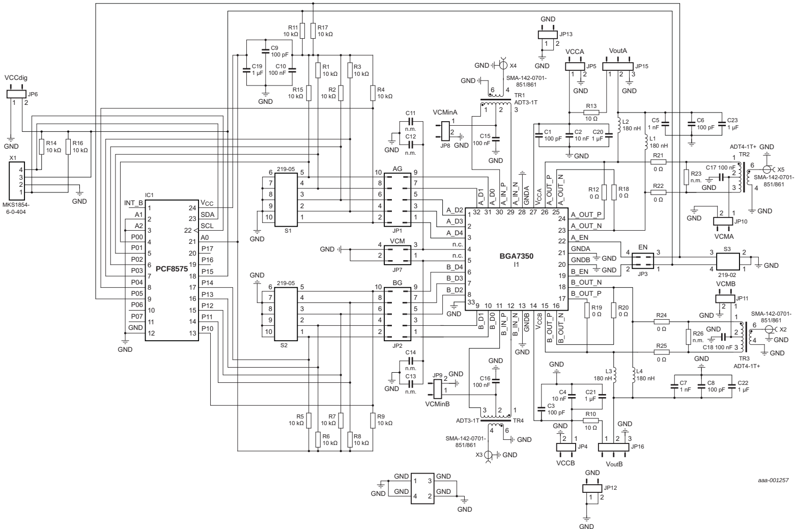
Fig 35. Schematic
