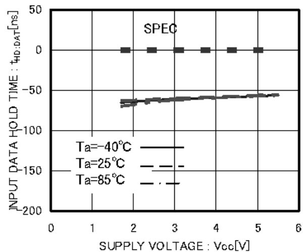
Figure 18. Input Data Hold Time t_{HD:DAT}(LOW)
