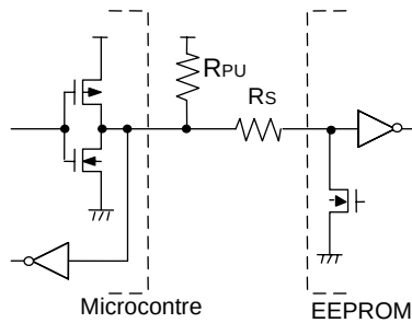
Figure 49. I/O circuit
