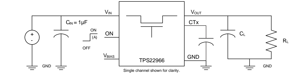
Test Circuit
