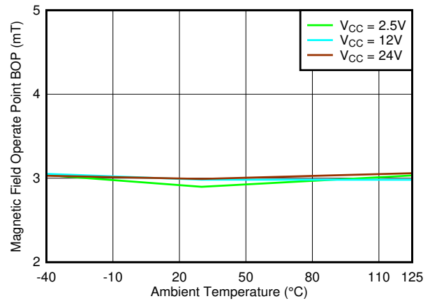
Figure 7-40. B OP_Z Threshold vs. Temperature
