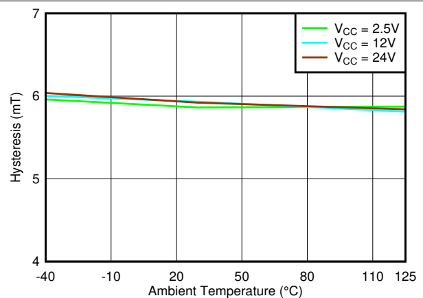
Figure 7-44. Hysteresis Z vs. Temperature
