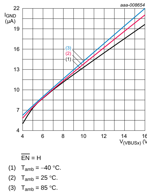
Fig 9. Ground current versus input voltage on pin VBUSI
