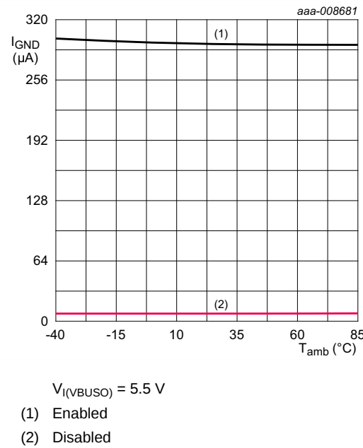
Fig 7. Ground current versus temperature
