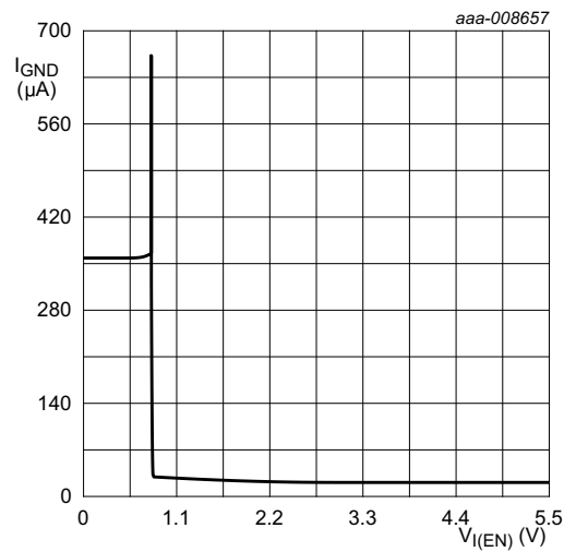
Fig 12. Ground current versus input voltage on pin EN
