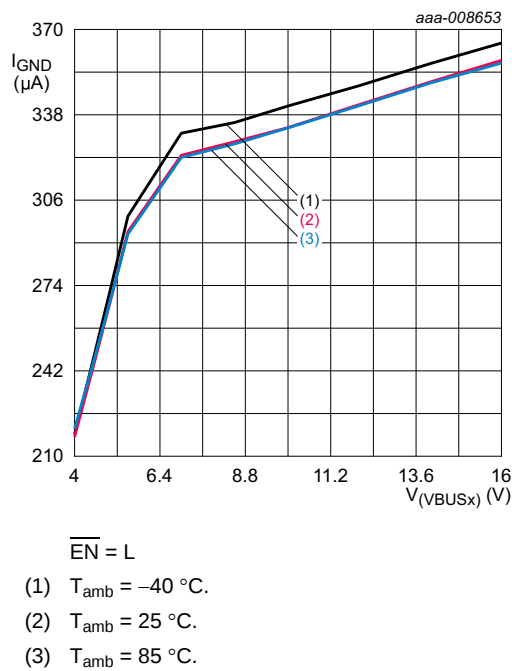
Fig 8. Ground current versus input voltage on pin VBUSI
