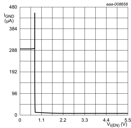
Fig 13. Ground current versus input voltage on pin EN
