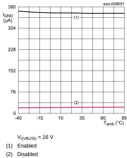
Fig 6. Ground current versus temperature
