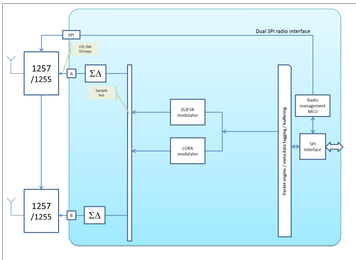
Figure 15: Transmission Schematics
