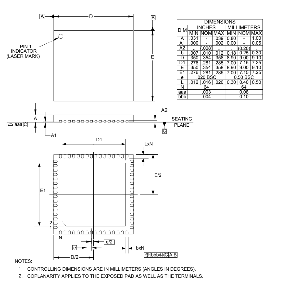
Figure 18: Package Dimensions
