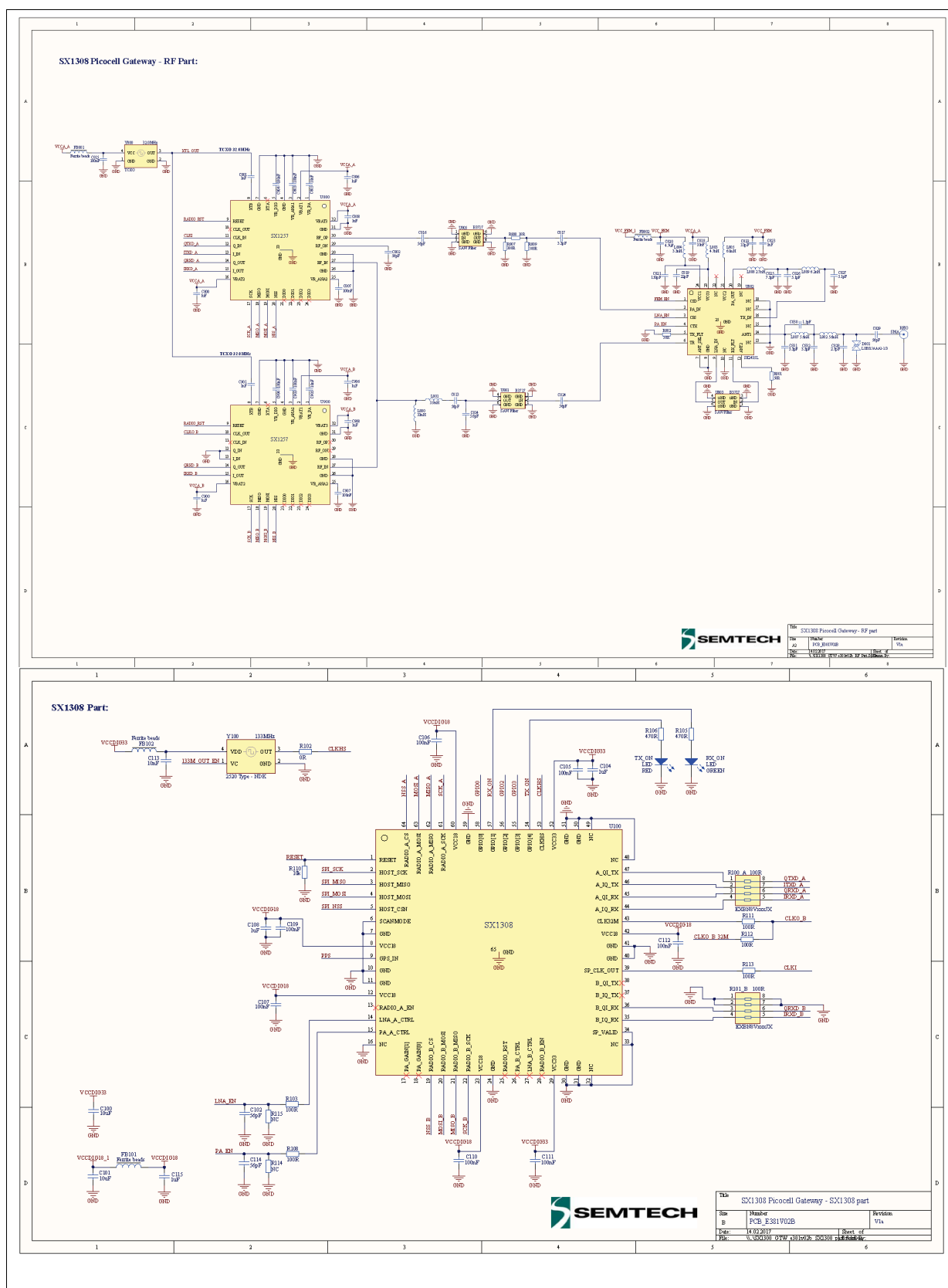
Figure 16: Reference Application
