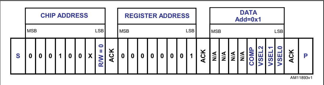
Figure 10. Example of writing procedure starting with first data address 0x2
