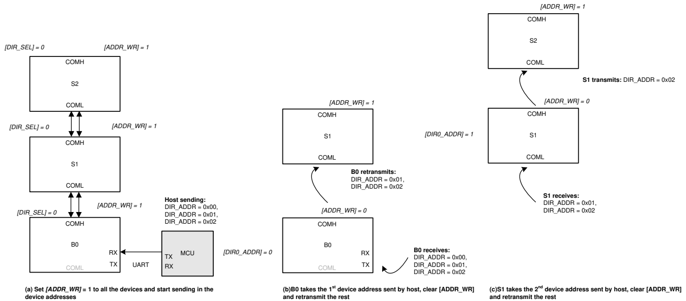
Figure 8-36. Auto-Addressing
