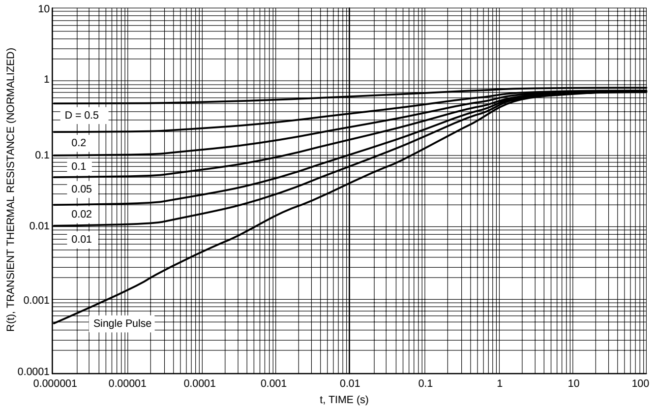
Figure 13. Thermal Response
