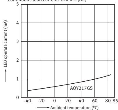
5-2. LED operate current vs. ambient temperature characteristics
