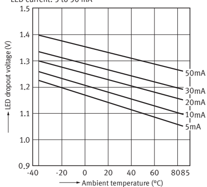
7-1. LED dropout voltage vs. ambient temperature characteristics
