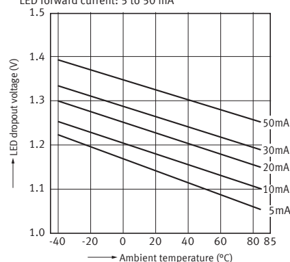
7-2. LED dropout voltage vs. ambient temperature characteristics
