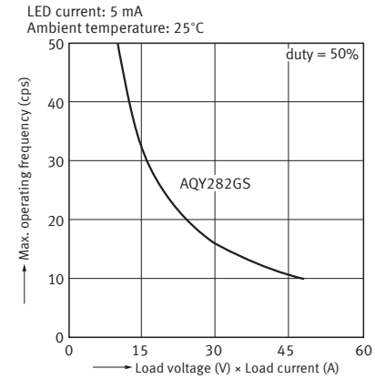
13-1. Maximum switching frequency vs. load voltage and load current
