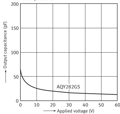
12-1. Output capacitance vs. applied voltage characteristics
