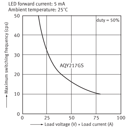
13-2. Maximum switching frequency vs. load voltage and load current
