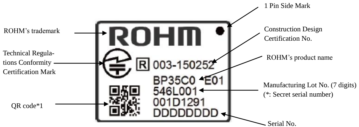
Fig. 4. Marking Specification
