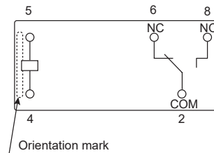
Schematics (FTR-K1CK( )W-MA) (BOTTOM VIEW)
