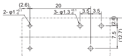
PC board mounting hole layout (FTR-K1CK( )W-MA) (BOTTOM VIEW)
