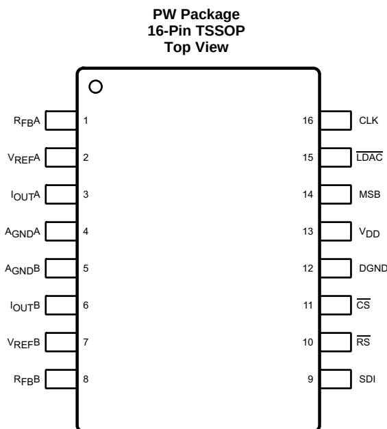
Pin Functions
