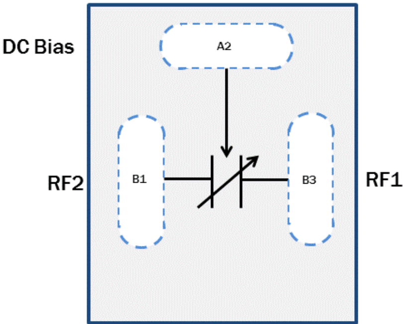
Figure 1. PTIC Functional Block Diagram (Top View)
