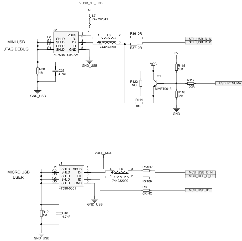
Figure 10. STEVAL-ST25R3916B main board circuit schematic (9 of 10)
