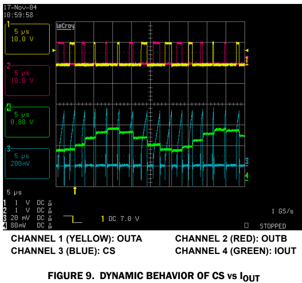
Figure 8 shows the relationship between the CS signal and IOUT under steady state conditions. IOUT is 4x the average of CS. Figure 9 shows the dynamic behavior of the current averaging circuitry when CS is modulated by an external sine wave. Notice IOUT is updated by the sample and hold circuitry at the termination of the active output pulse.
