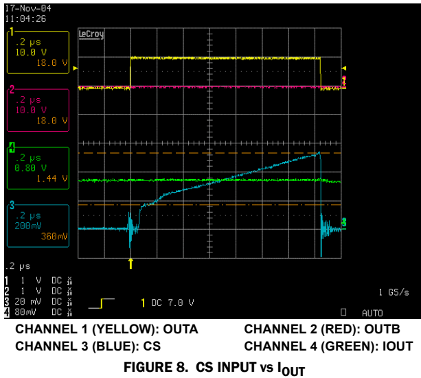
Figure 8 shows the relationship between the CS signal and IOUT under steady state conditions. IOUT is 4x the average of CS. Figure 9 shows the dynamic behavior of the current averaging circuitry when CS is modulated by an external sine wave. Notice IOUT is updated by the sample and hold circuitry at the termination of the active output pulse.
