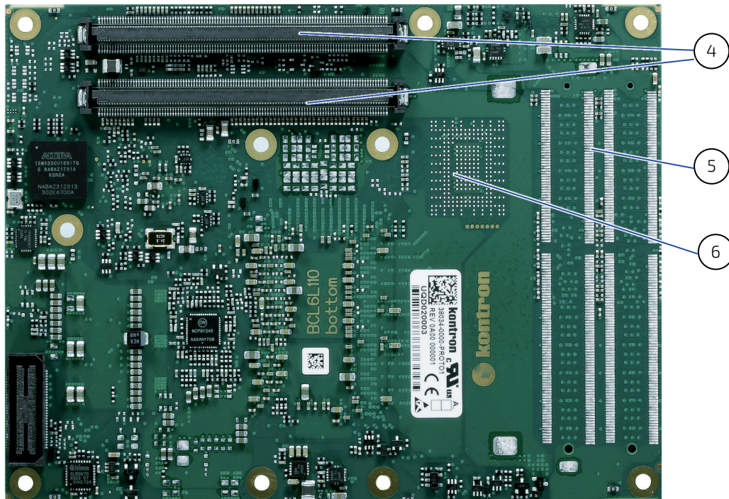
Figure 3: Bottom View COMe-bCL6
