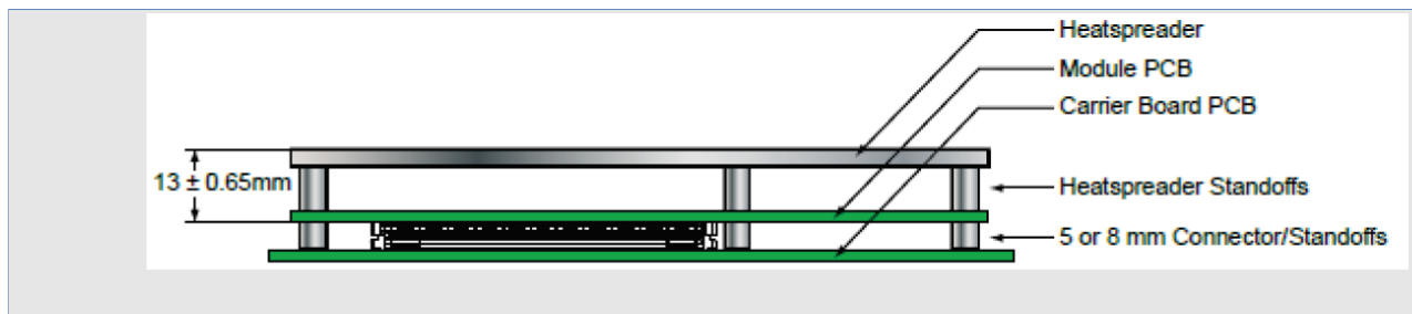
Figure 6: Module Height
