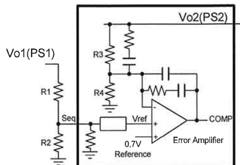
Figure 12 Tracking Diagram
