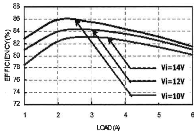
Figure 47 :Converter efficiency vs. output current(1.2V out)
