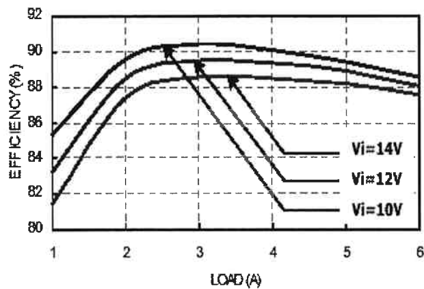
Figure 46 :Converter efficiency vs. output current(2.5V out)
