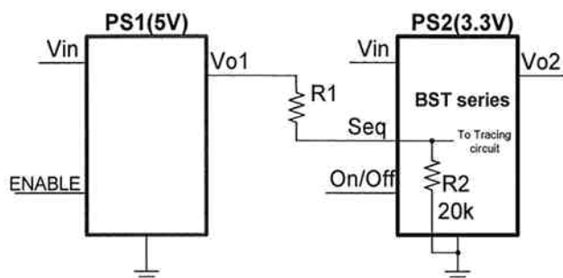
Figure 16 Ratio-Metric tracking connection method
