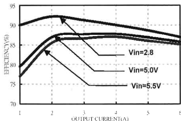
Figure 41 :Converter efficiency vs. output current(1.2V out)
