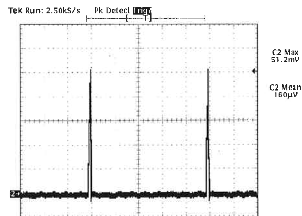
Figure 63 : Typical transient response to step load change at 2.5A/μS from 50% to 100% of I_o , max at 12Vin, 5.0V out (Cout=1μceramic, 10μF tantalum)
