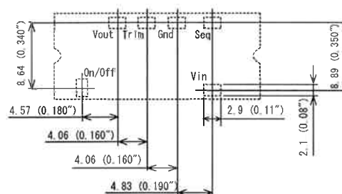
Figure 2 Recommended PWB PAD LAYOUT (Top View)
