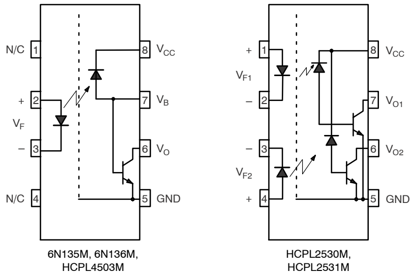
Figure 1. Schematics
