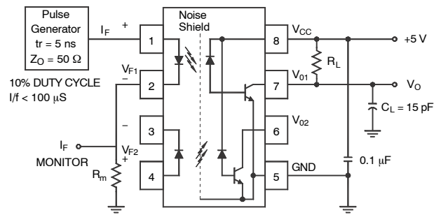
Test Circuit for HCPL2530M and HCPL2531M
