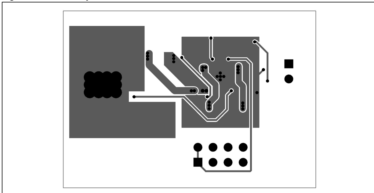
Figure 7. Bottom layer
