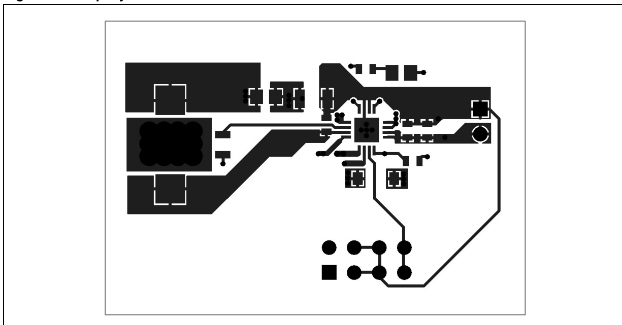
Figure 6. Top layer
