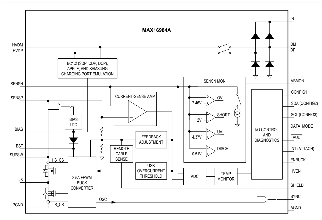
Figure 1. Detailed Block Diagram
