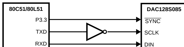
Figure 42. 80C51/80L51 Interface
