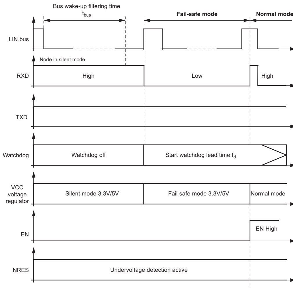
Figure 4-3. LIN Wake Up from Silent Mode
