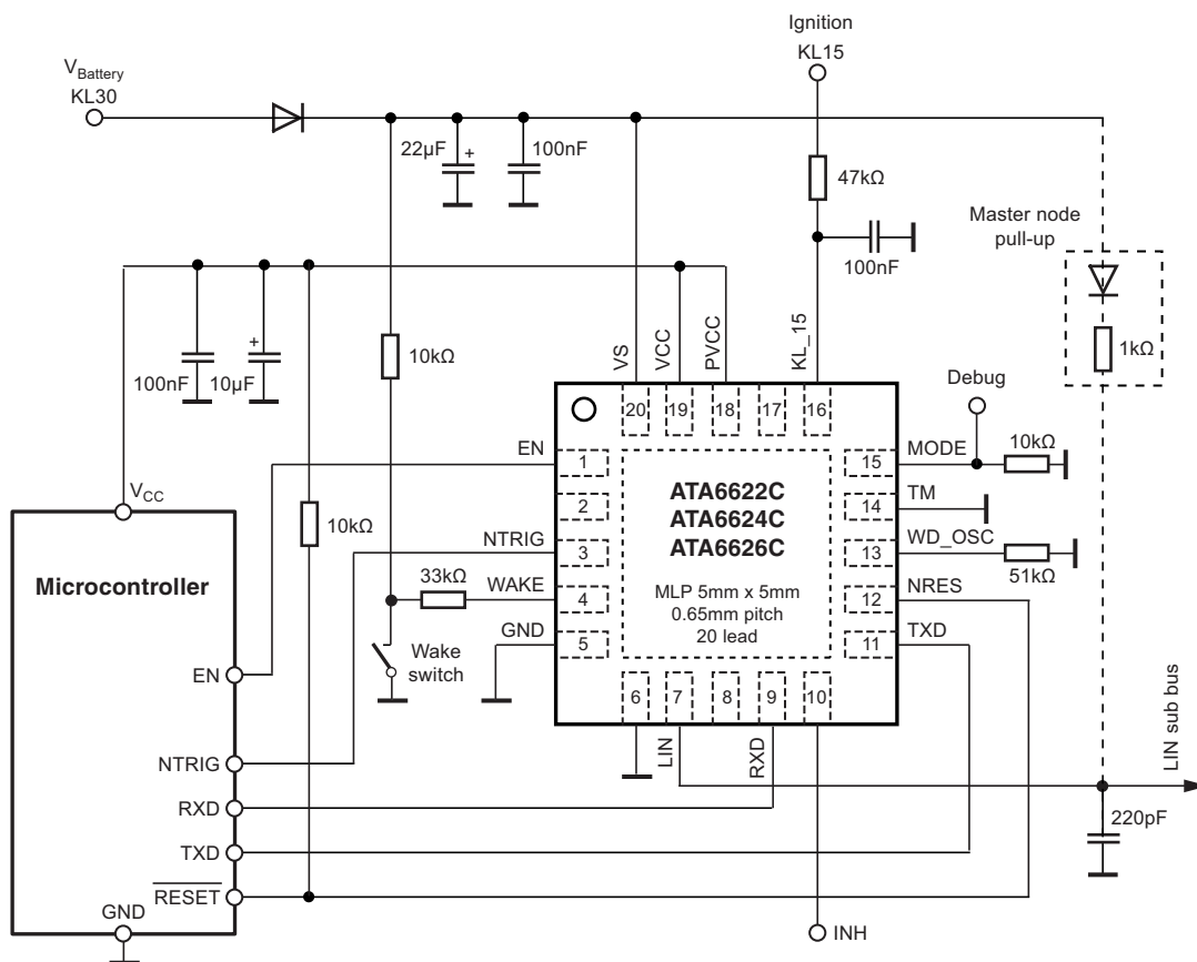
Figure 9-2. Typical Application Circuit
