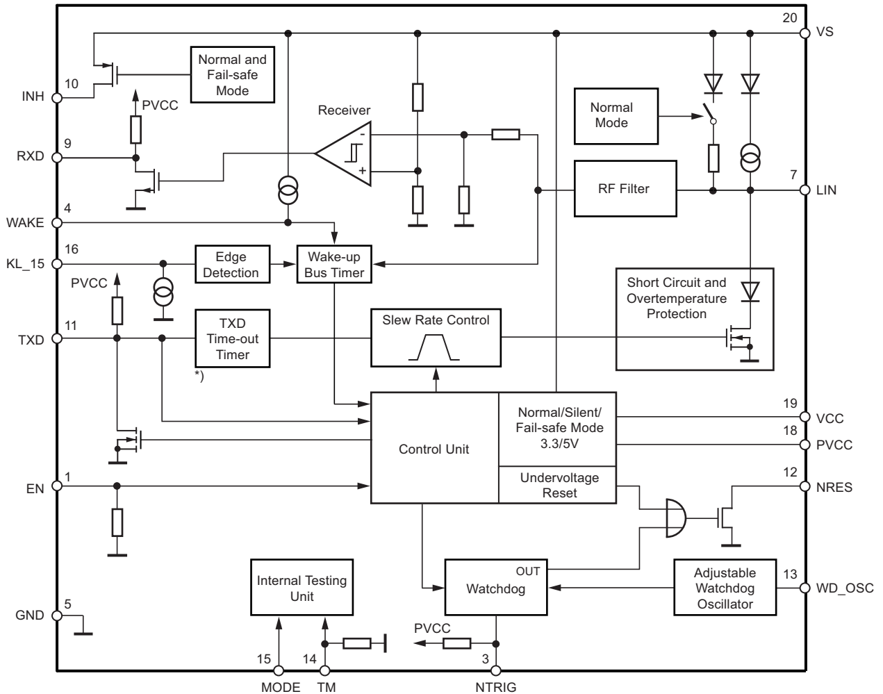
Figure 1-1. Block Diagram
