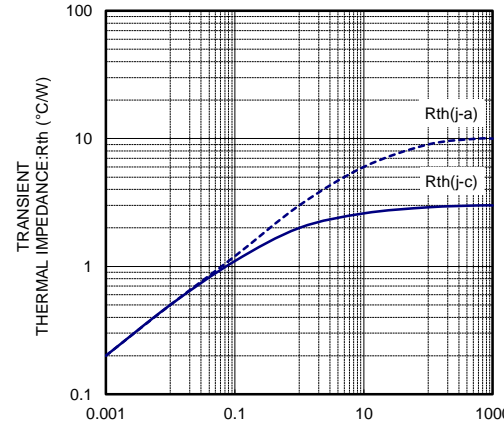
R_th-t CHARACTERISTICS
