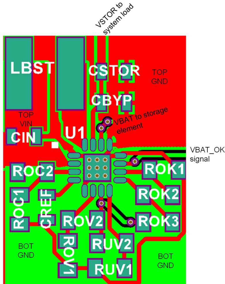
Figure 11-1. Recommended Layout
