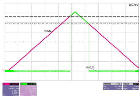
Figure 9-5. MPPT Operation
