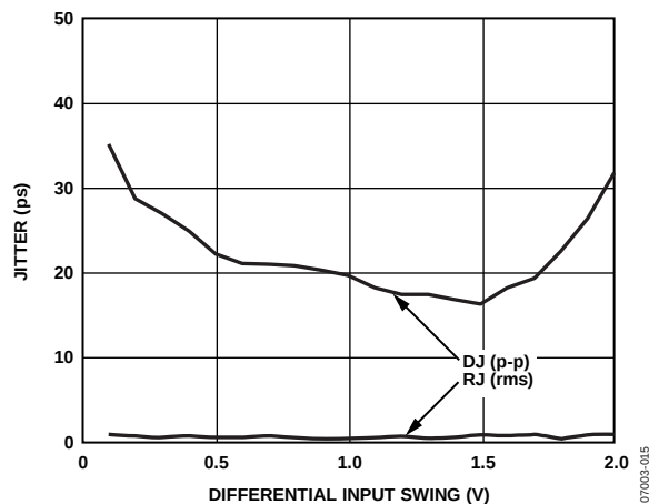
Figure 14. Jitter vs. Differential Input Swing
