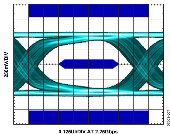
Figure 7. Rx Eye Diagram at TP3 (Cable = 2 m, 30 AWG)
