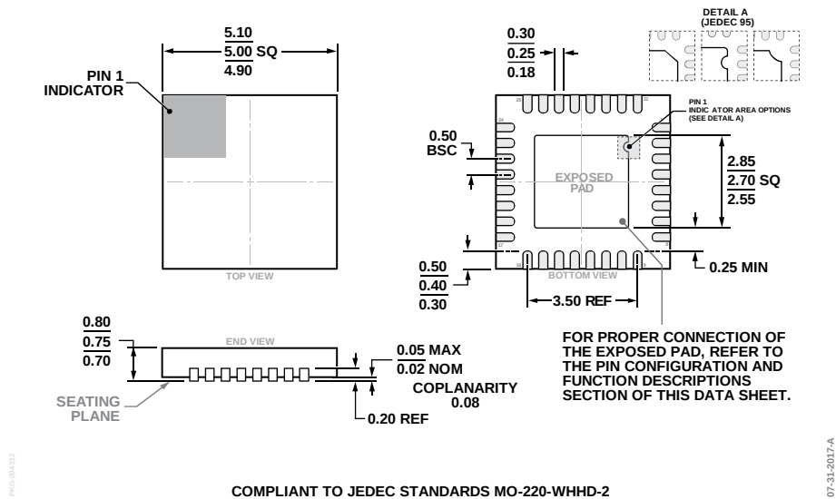
COMPLIANT TO JEDEC STANDARDS MO-220-WHHD-2 Figure 27. 32-Lead Lead Frame Chip Scale Package [LFCSP] 5 mm × 5 mm Body and 0.75 mm Package Height (CP-32-21) Dimensions shown in millimeters
