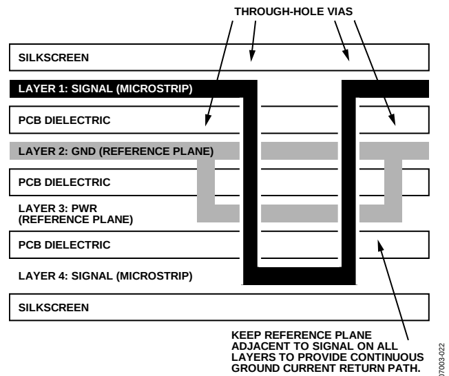
Figure 21. Example Routing of Reference Plane
