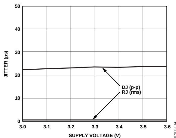
Figure 13. Jitter vs. Supply Voltage
