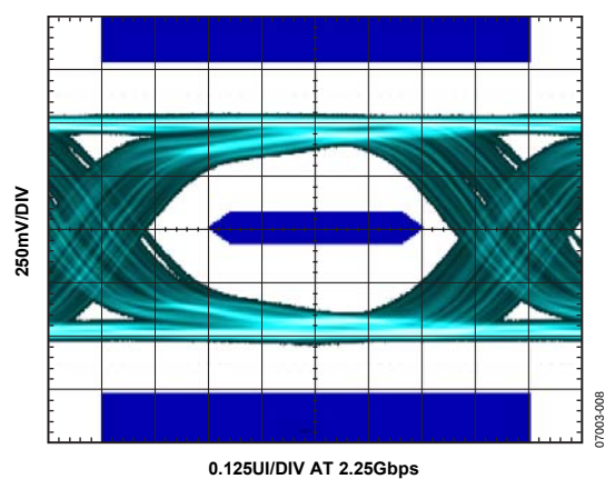
Figure 8. Rx Eye Diagram at TP3 (Cable = 6 m, 24 AWG)
