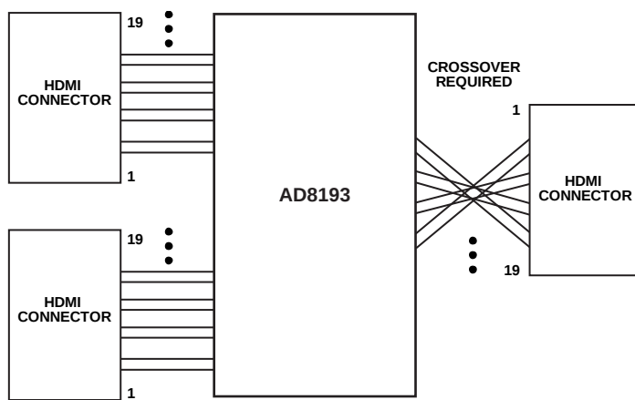
Figure 24. Block Diagram of AD8193 Evaluation Board Showing Output Crossover
