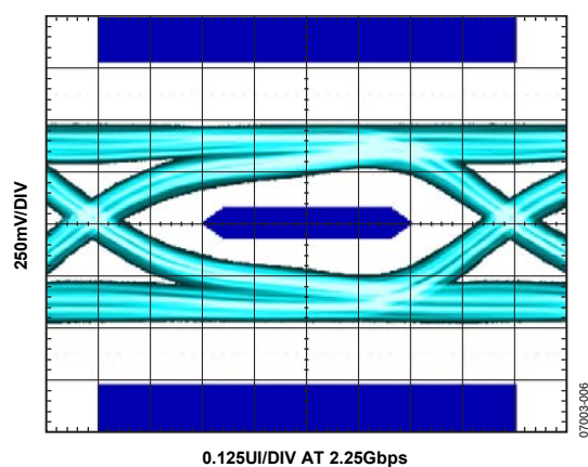
Figure 6. Rx Eye Diagram at TP2 (Cable = 6 m, 24 AWG)
