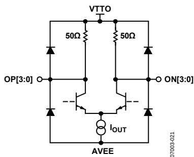
Figure 20. High Speed Output Simplified Schematic
