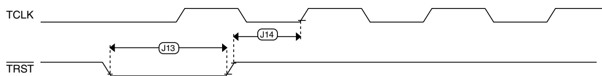
Figure 10. \overline{\text{TRST}} timing
