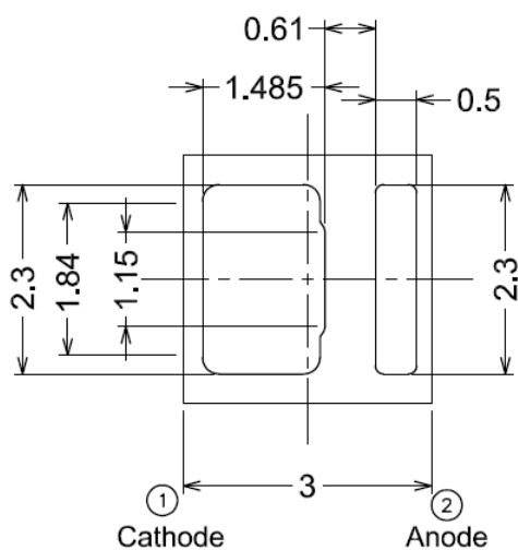
Bot. view
