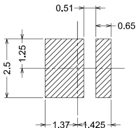
Soldering patterns
