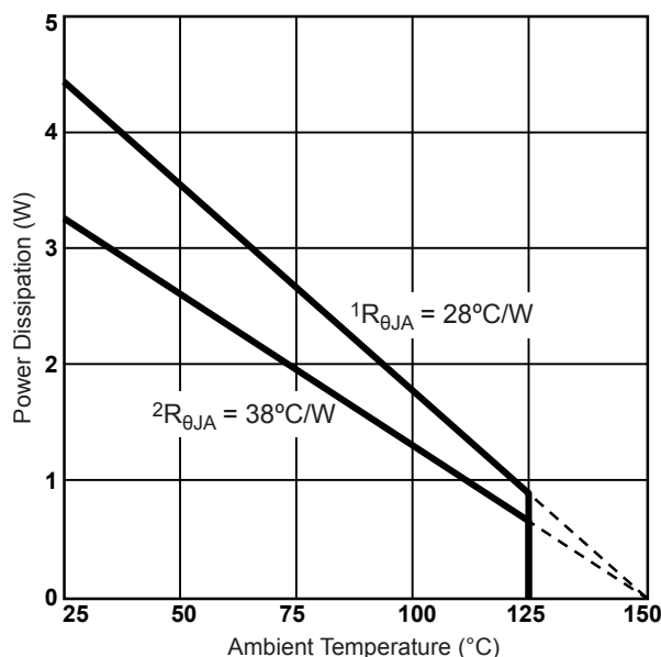
Allowable Package Power Dissipation
