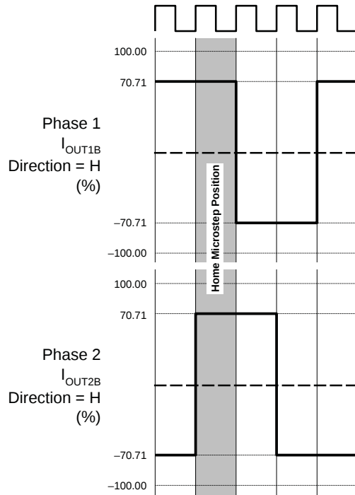
Figure 5. Full Step
