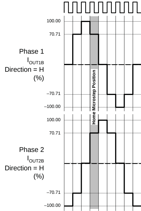
Figure 6. Half Step
