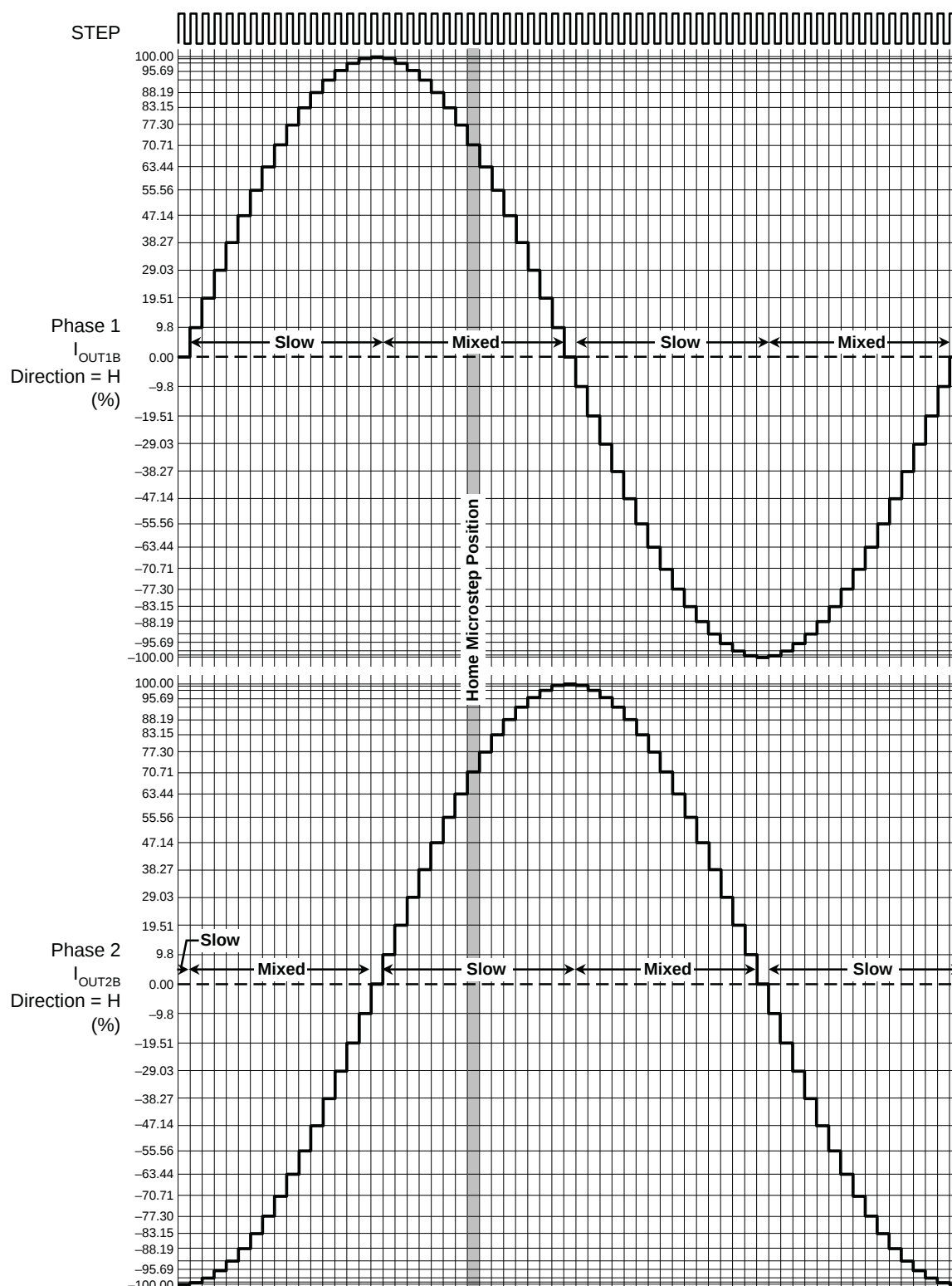
Figure 8. Sixteenth Steps
