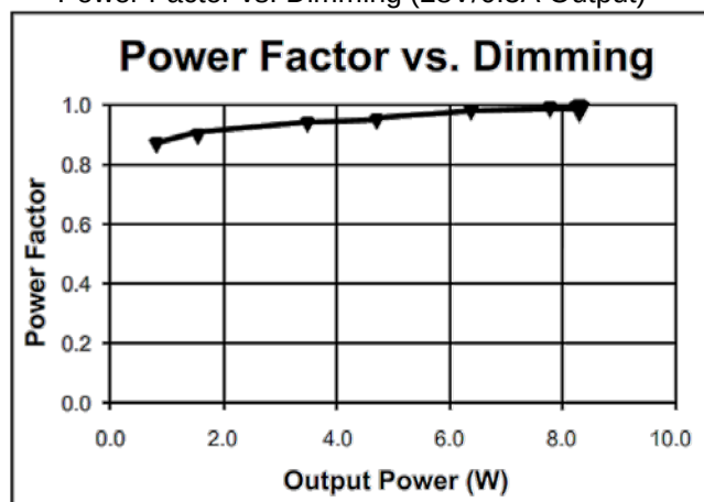
Power Factor vs. Dimming (28V/0.3A Output)
