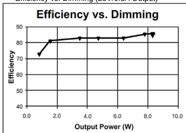
Efficiency vs. Dimming (28V/0.3A Output)
