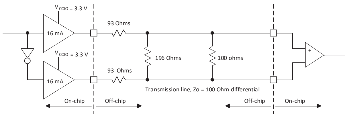
Figure 3.3. Differential LVPECL
