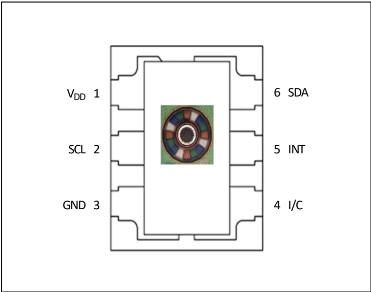
Figure 3: Pin Diagram
