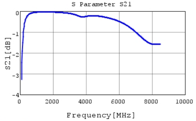
GRM1885C1H150JA01 S21 DCOV, 25degC
