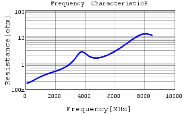
GRM1885C1H150JA01 R DCOV, 25degC
