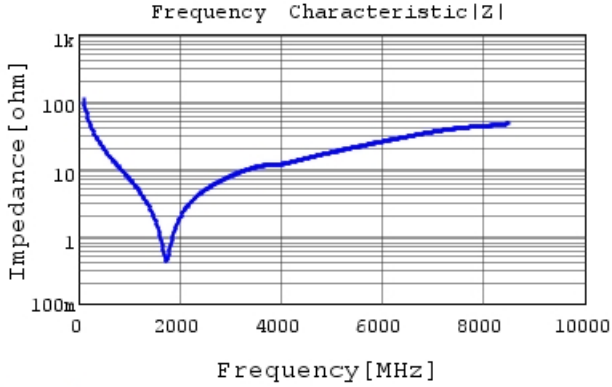
GRM1885C1H150JA01 |Z| DCOV, 25degC
