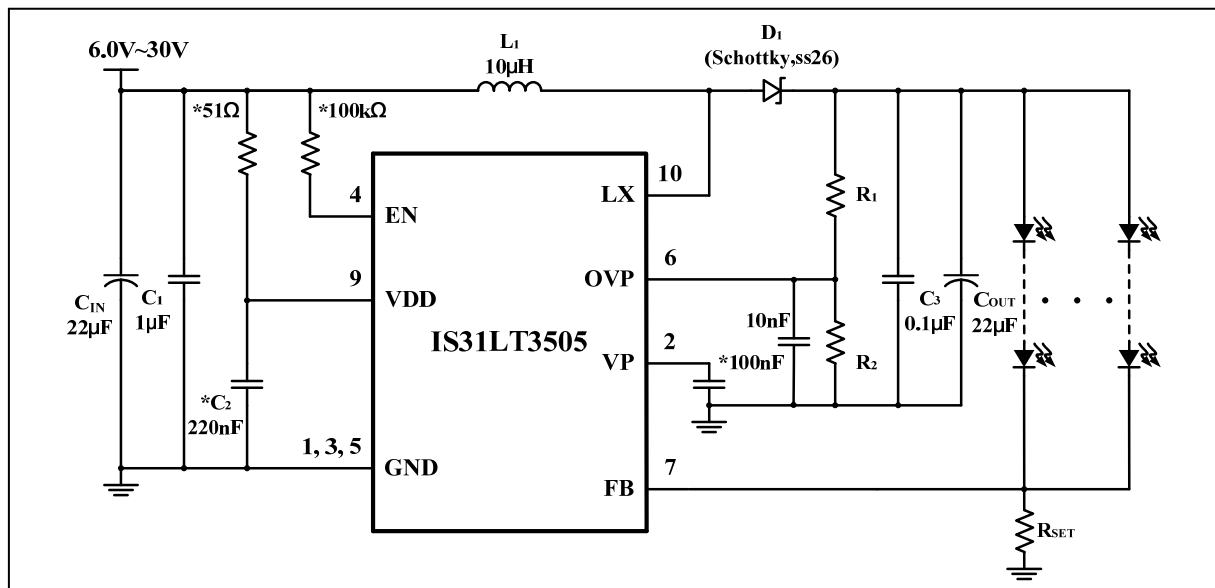
Figure 1 Typical Application Circuit (Constant Current to Drive White LEDs)
