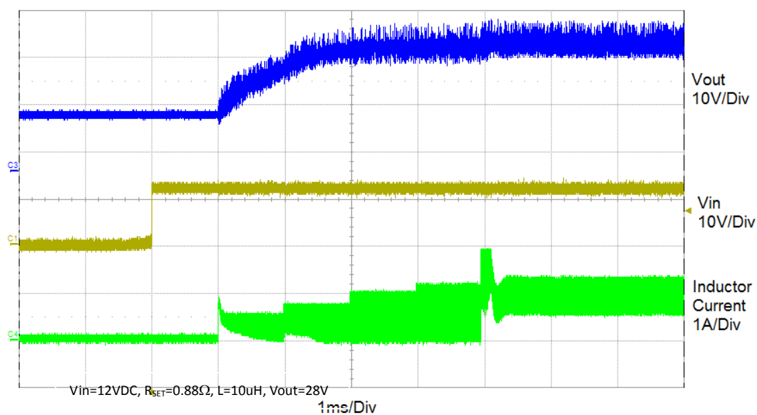
Figure 11 Soft-start waveform
