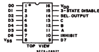
TERMINAL ASSIGNMENT
