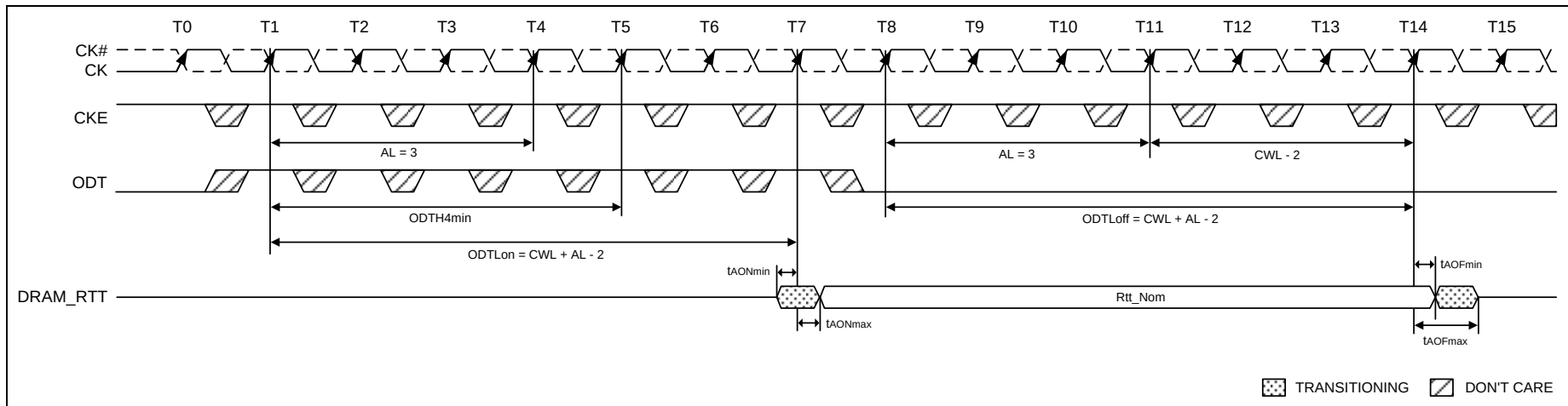
Figure 74 – Synchronous ODT Timing ( AL = 3 ; CWL = 5 ; ODT_{on} = AL + CWL - 2 = 6 ; ODT_{off} = AL + CWL - 2 = 6 )
