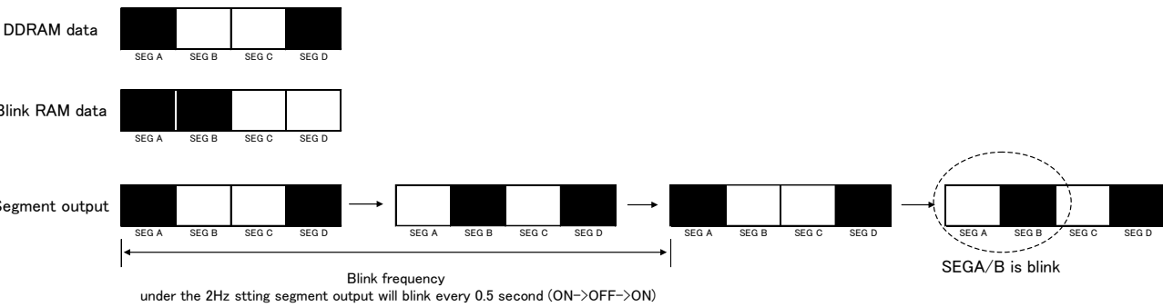
Figure 17. Blink Operation
