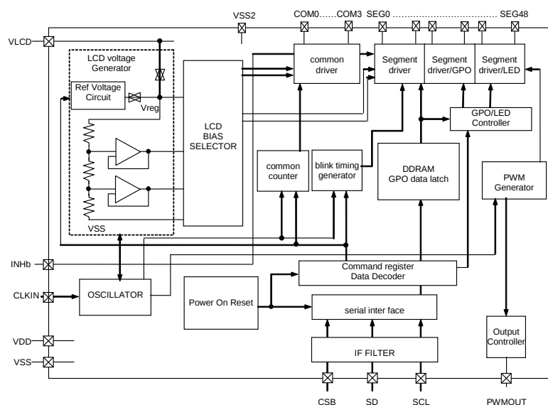
Figure 6. Block Diagram
