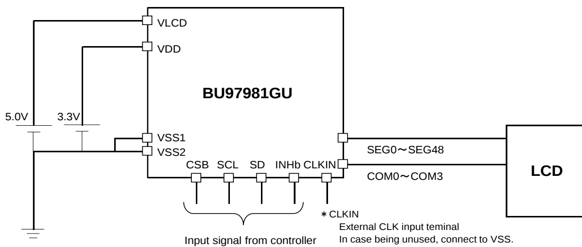
Figure 14. BU97981GU E.g. of Recommended Circuit
